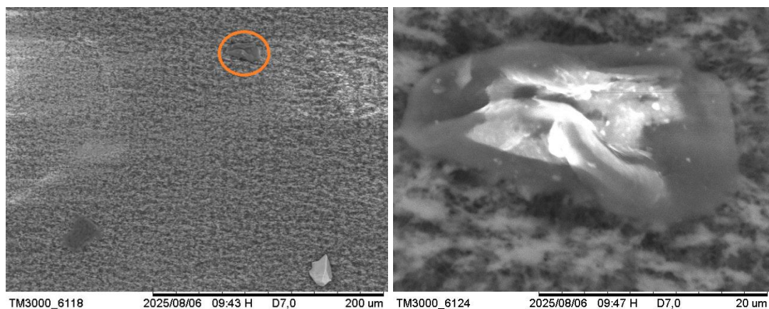
Figure 1. Description of Microplastics in bottled drinking water heated within 4 hours with a temperature of 60°C. 200μm magnification (left) and 20μm magnification (right).
